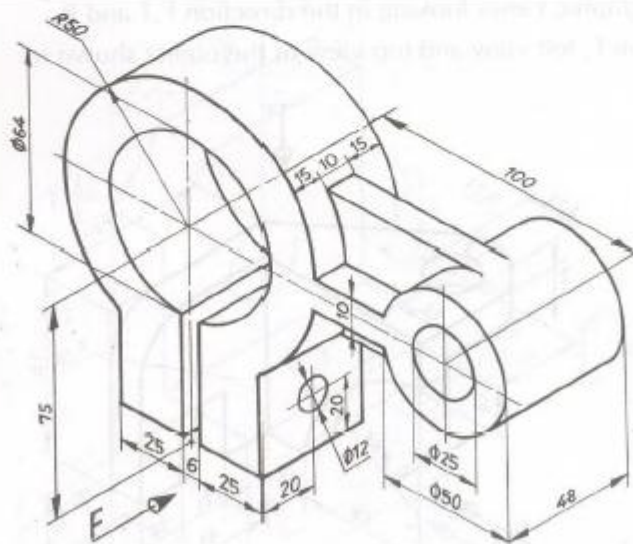
Cast iron Block
